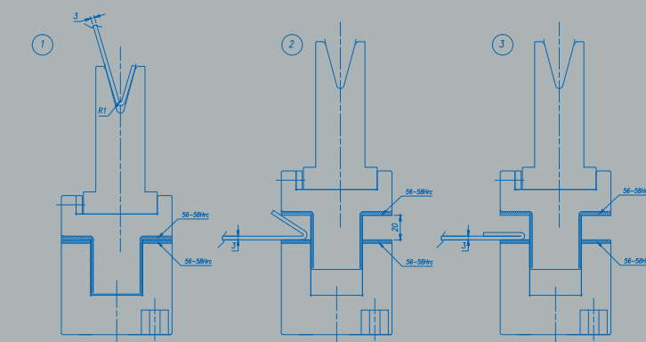
Special hemming table, pneumatically driven.
