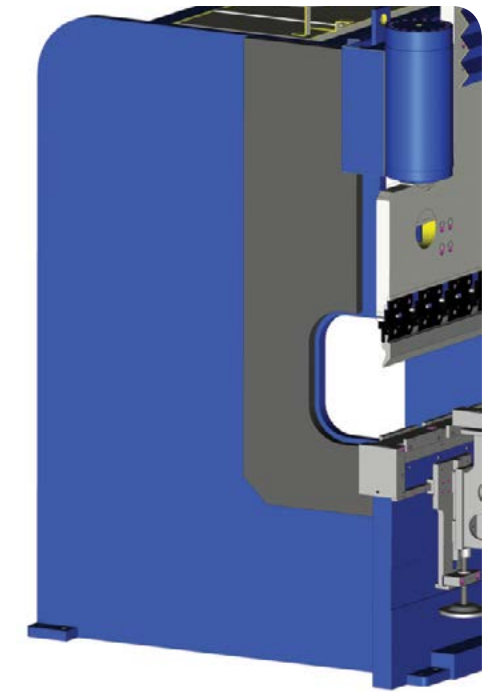
Extra external welded-steel side frame to increase machine's rigidity and minimize deformation.
